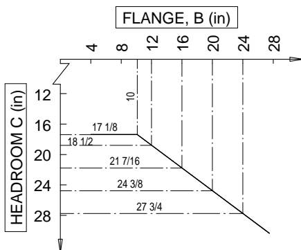
HEADROOM CHART
