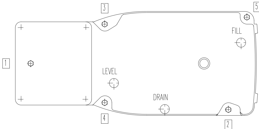
Figure 1 – Frame 2 Bolt-tightening Sequence
